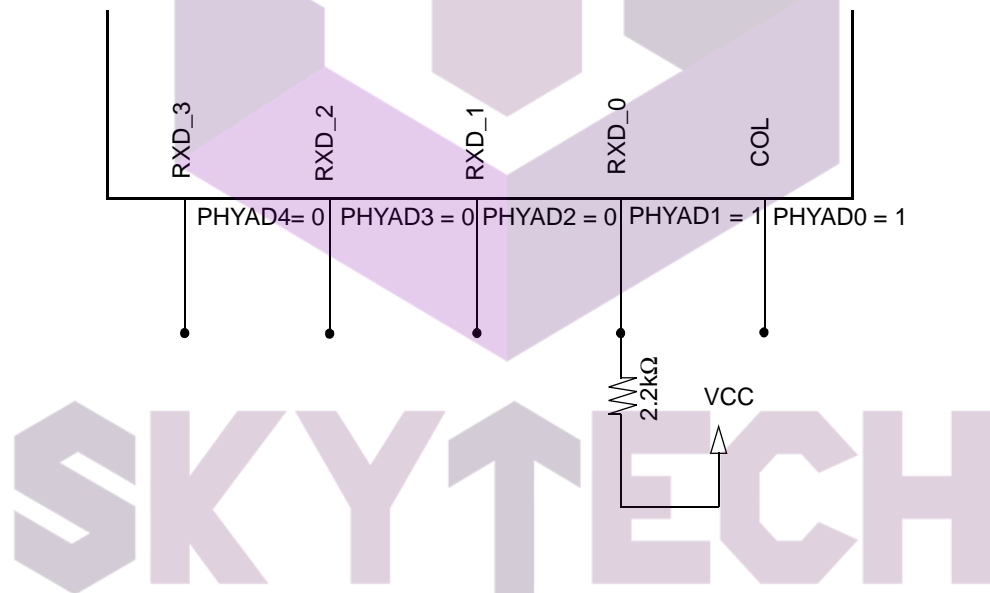
Figure 2. PHYAD Strapping Example
